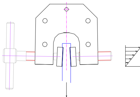
SP154 deformation and rotation of jaws under load
